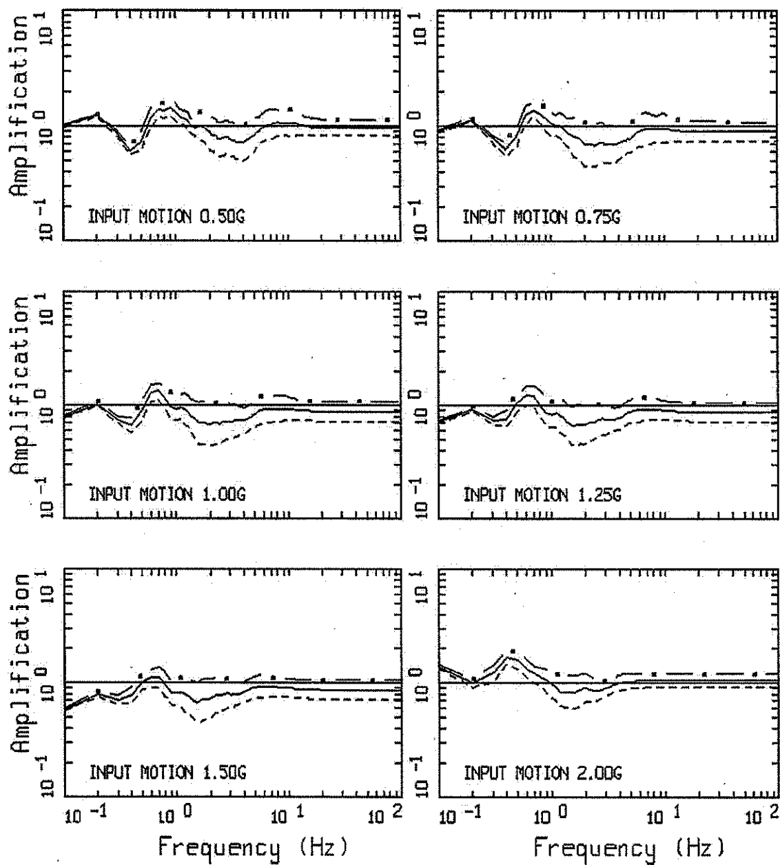
AMPLIFICATION, TA-55 WNA: PAGE 2 OF 3 STOEK 04 UNADJUSTED CURVES, HORIZONTAL
