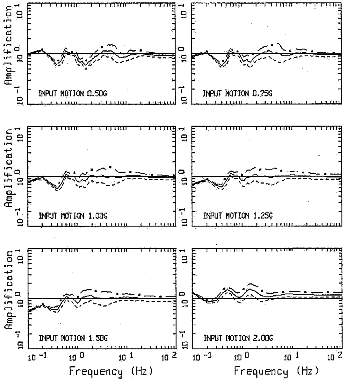
AMPLIFICATION, TA-16 WNA: PAGE 2 OF 3 STOKOE 04 ADJUSTED CURVES, HORIZONTAL
