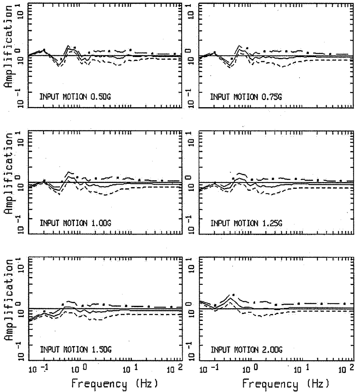
AMPLIFICATION, TA-D3 WNA: PAGE 2 OF 3 STOKOE D4 ADJUSTED CURVES, HORIZONTAL
